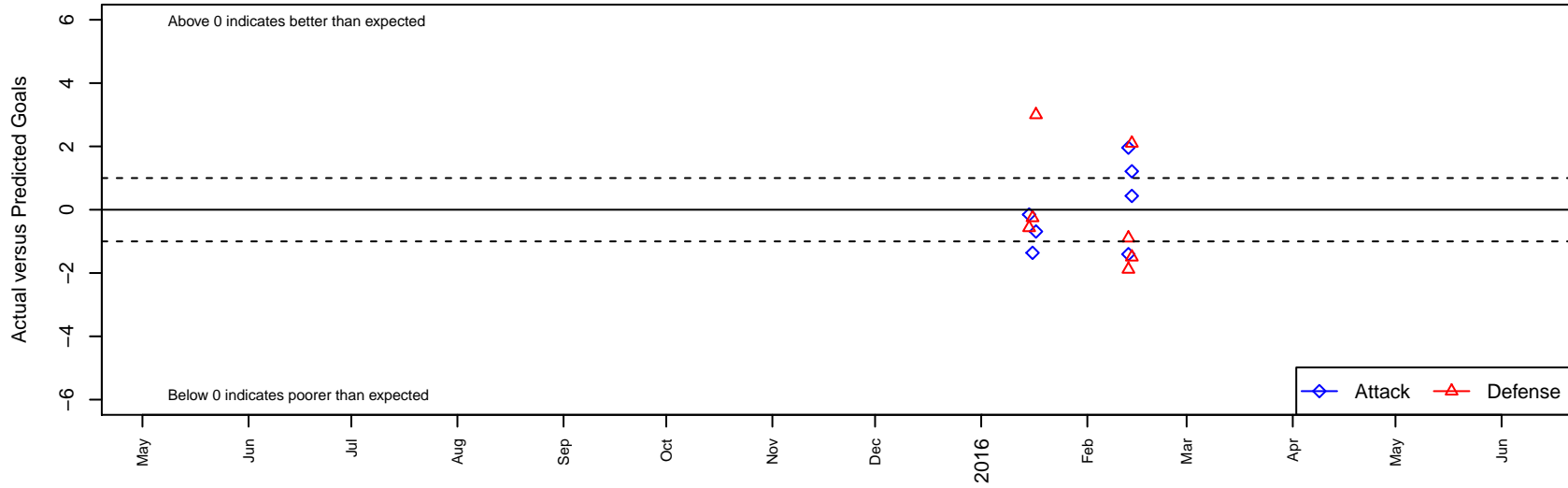
Real Henderson Black B98 Dots are actual minus expected GF (blue circles) and GA (red triangles). Blue line is smoothed change in attack strength. Red is smoothed change in defense strength.
